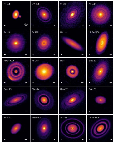
ALMA DSHARP 240 GHz continuum images of 20 nearby disks. Reproduced from Andrews et al. (2018).
