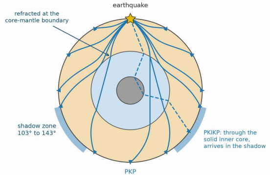
(b) P waves: refracted by the core
