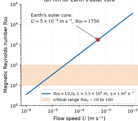
(b) R_m for Earth's outer core
