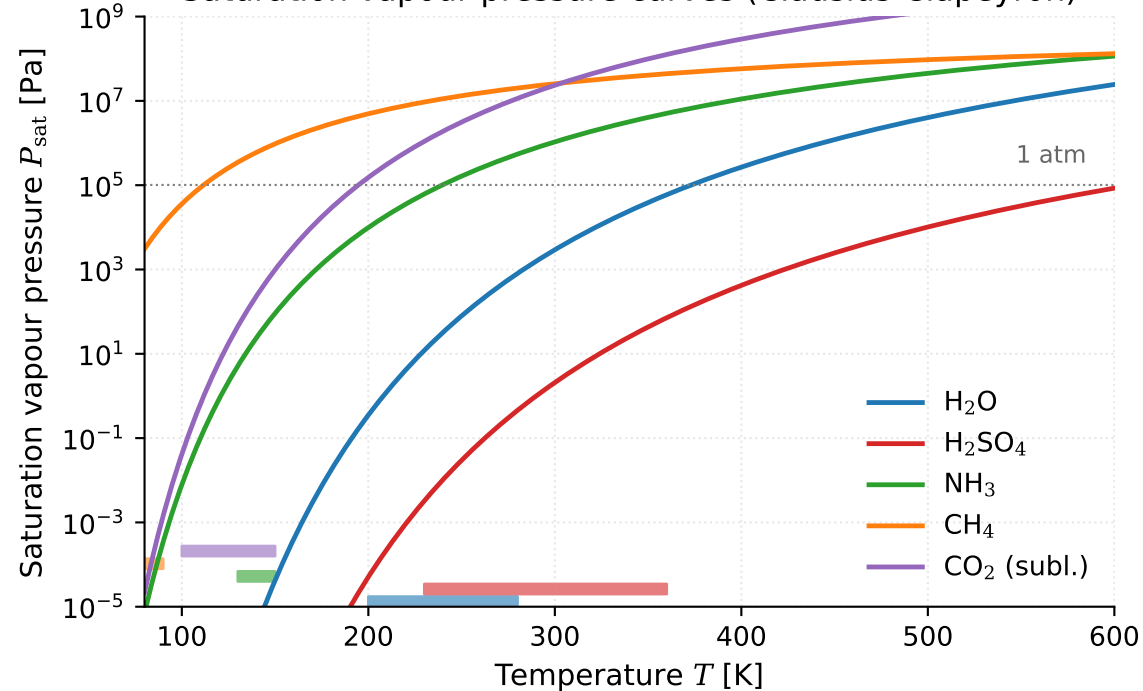
Saturation vapour pressure curves (Clausius-Clapeyron)
