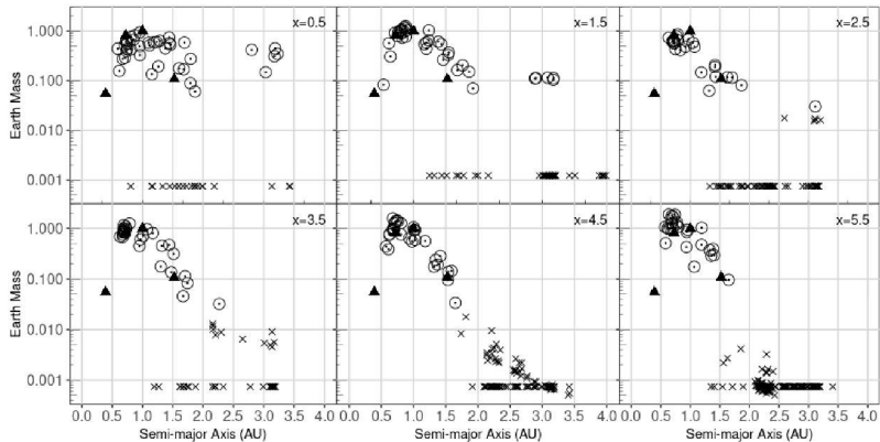
Remnant mass against semimajor axis in N-body terrestrial-formation simulations for surface-density slopes x = 0.5 – 5.5 ; triangles mark the real planets. Credit: Franco et al. (2022), Fig. A1.
