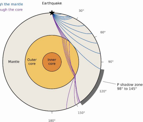
(a) P waves: refracted into the core
