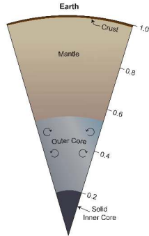
Earth's interior in cross-section. Credit: NASA/JPL-Caltech.
