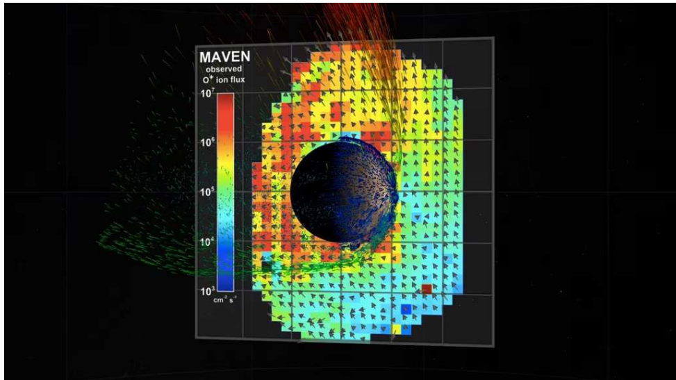
The ion plume escaping Mars, rendered from MAVEN data. Credit: NASA SVS.
