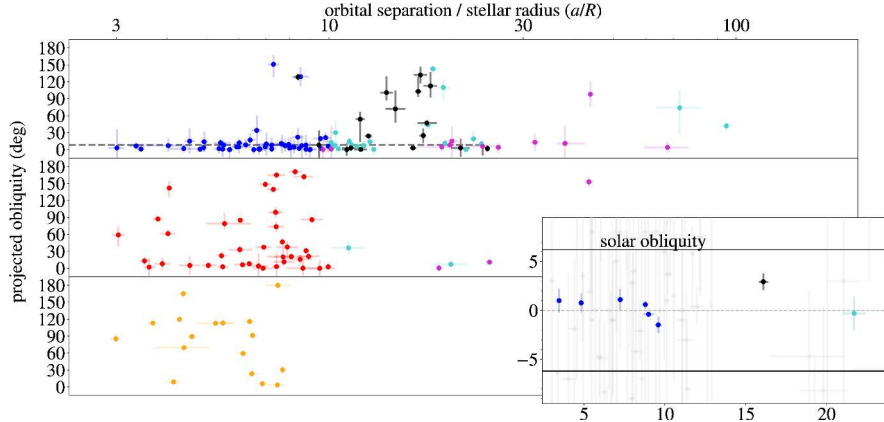
Observed stellar obliquities of hot Jupiter hosts against effective temperature and a/R_* . Albrecht et al. (2022).
