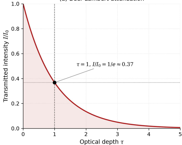
(a) Beer-Lambert attenuation
