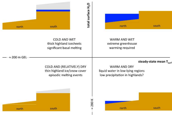
Long-term climate regimes of Mars: mean surface temperature (divider ~ 280 K) against surface H 2 O inventory (divider ~ 200 m GEL), with cross-sections. Credit: Wordsworth (2016), Fig. 7.
