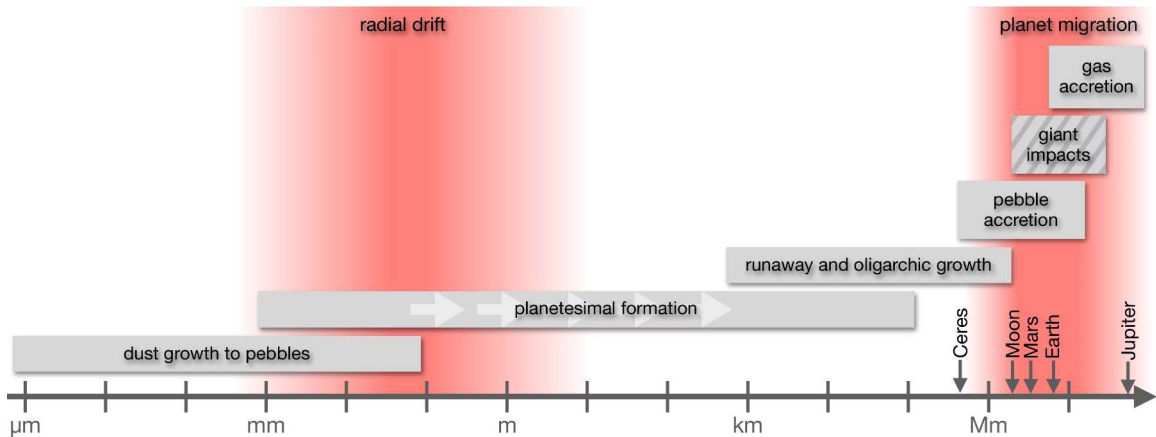
Roadmap of the planet-formation sequence, organised by body size. Adapted from Drążkowska et al. (2023).
