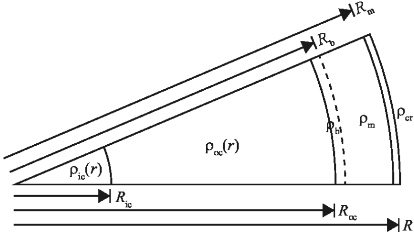
Mercury's layers from libration and gravity. Credit: Margot et al. (2018).
