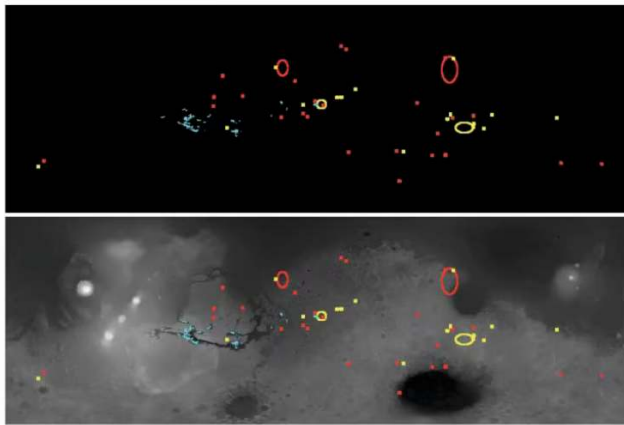
Global map of hydrated minerals from OMEGA: phyllosilicates (red), sulfates (blue) and other hydrated minerals (yellow). Credit: Bibring et al. (2006), Fig. 3.
