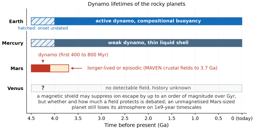
Dynamo lifetimes of the rocky planets. Course figure.
