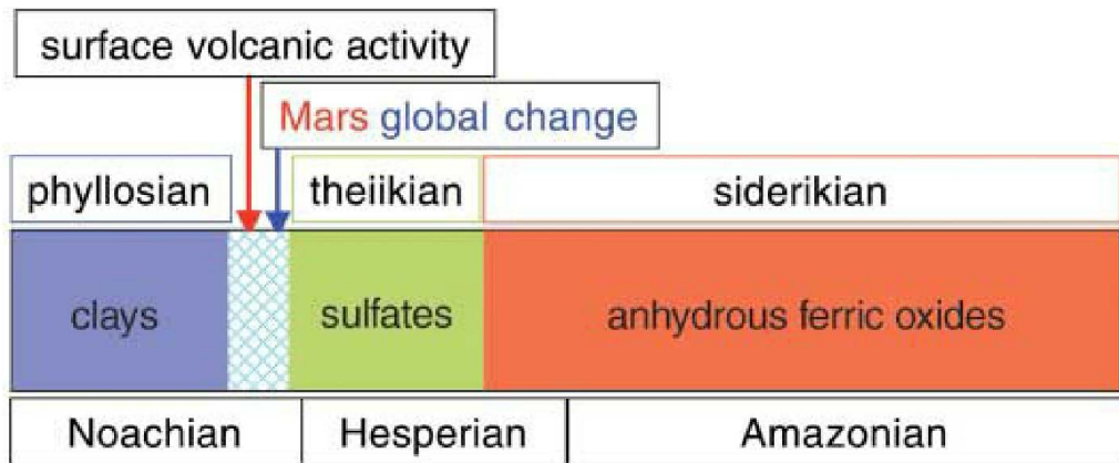
The OMEGA mineralogy time line. Credit: Bibring et al. (2006), Fig. 5.
