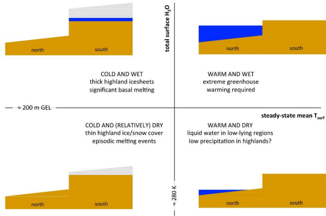
Climate regimes of Mars: \text{H}_2\text{O} inventory against surface temperature, with cross-sections. Credit: Wordsworth (2016), Fig. 7.
