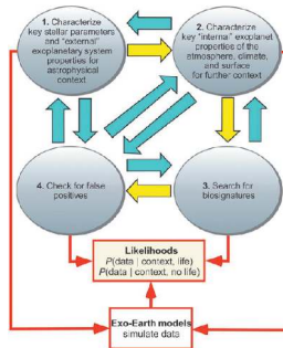
FIG. 2. Four components to assess whether exoplanet
