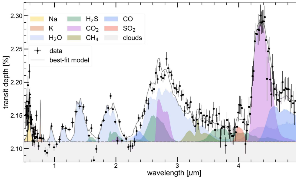
JWST/NIRSpec PRISM transmission spectrum of WASP-39 b: Na, K, \text{H}_2\text{O} , \text{CO} , \text{CO}_2 , \text{SO}_2 , \text{CH}_4 , clouds. Rustamkulov+ 2023.
