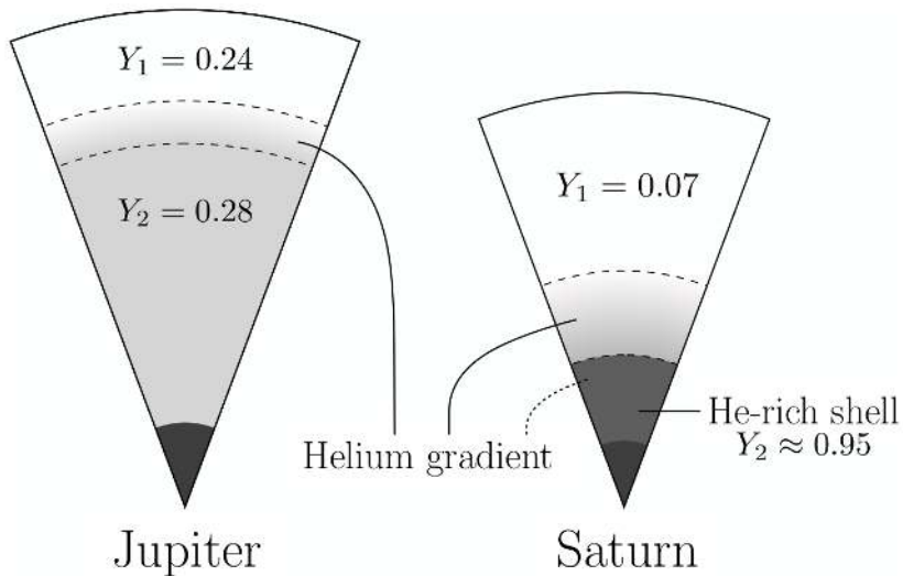
Helium phase separation in Jupiter and Saturn. Credit: Mankovich & Fortney (2020), Fig. 3.
