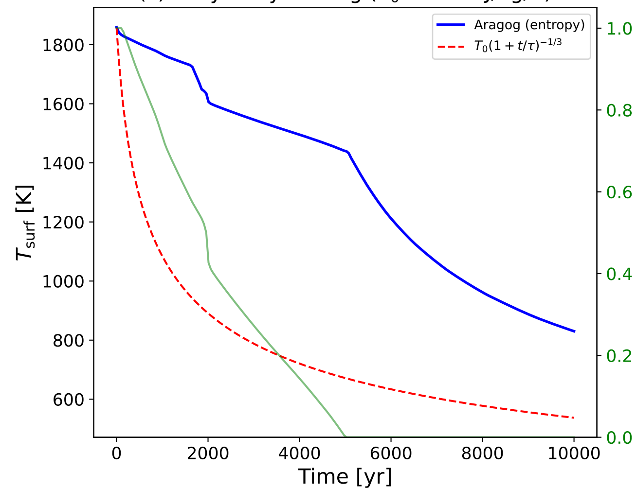
(c) Grey-body cooling ( S_0 = 3200 J/kg/K)
