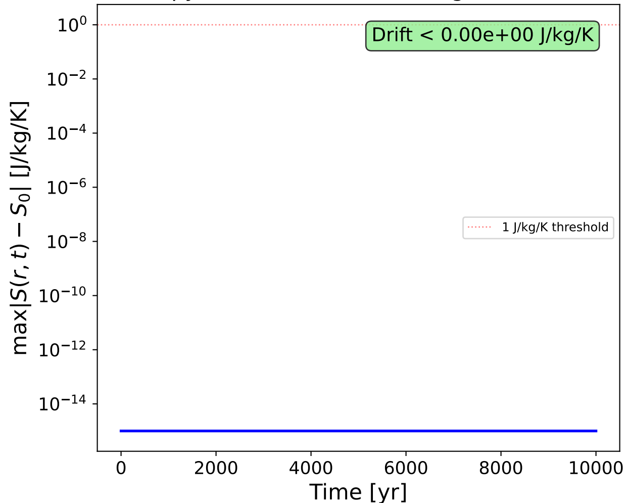
(c) Grey-body cooling ( S_0 = 3200 J/kg/K)
