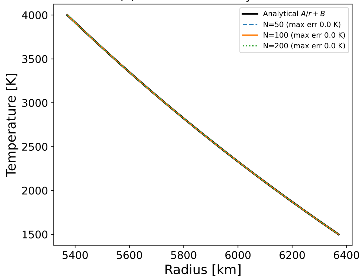
(a) Conduction steady state
