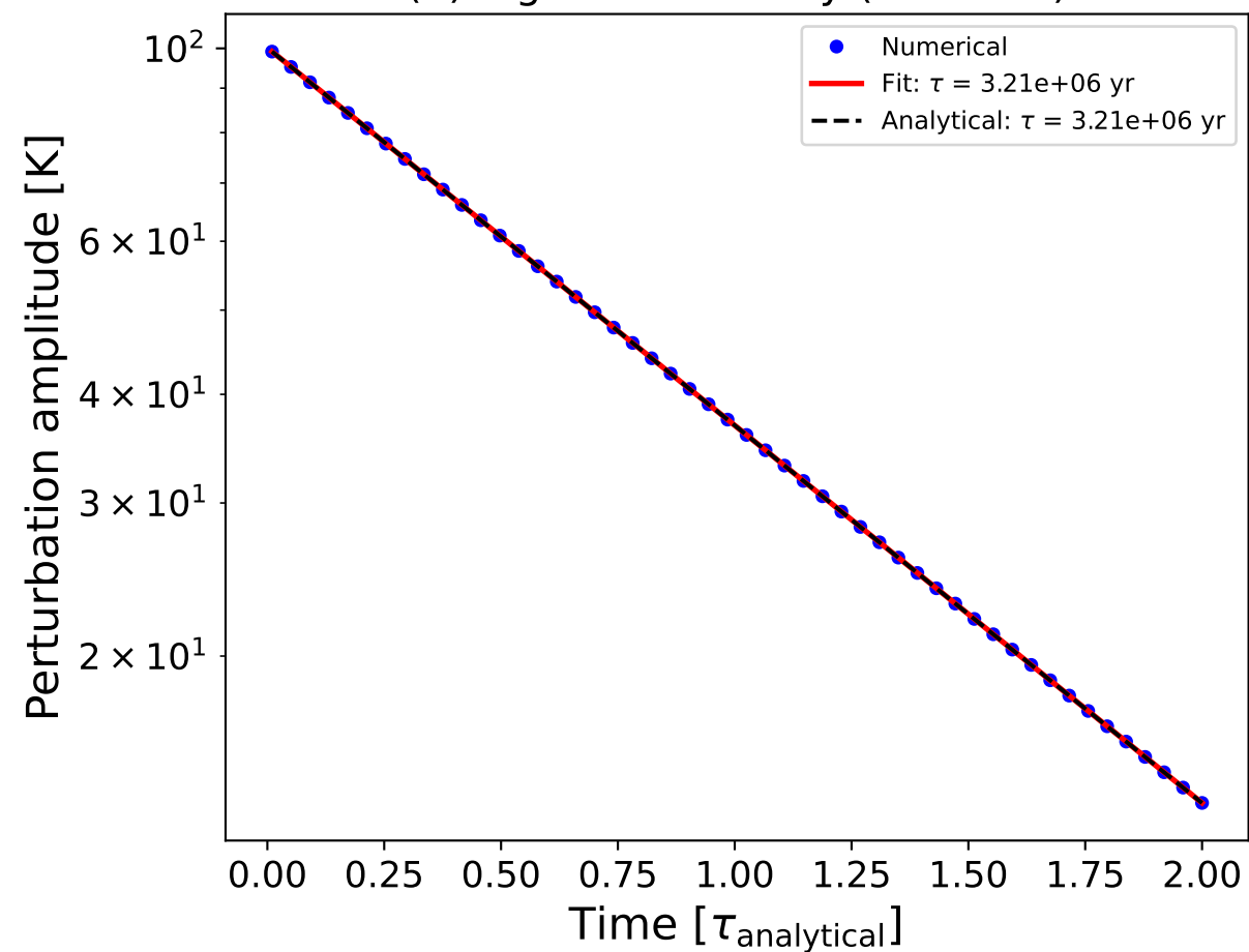
(b) Eigenvalue decay (0% error)
