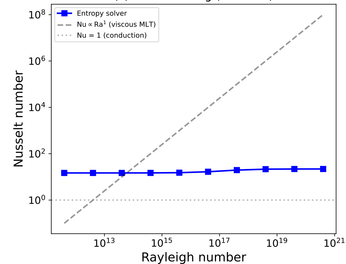
(c) Nu-Ra scaling ( \alpha = 10^{-5} )
