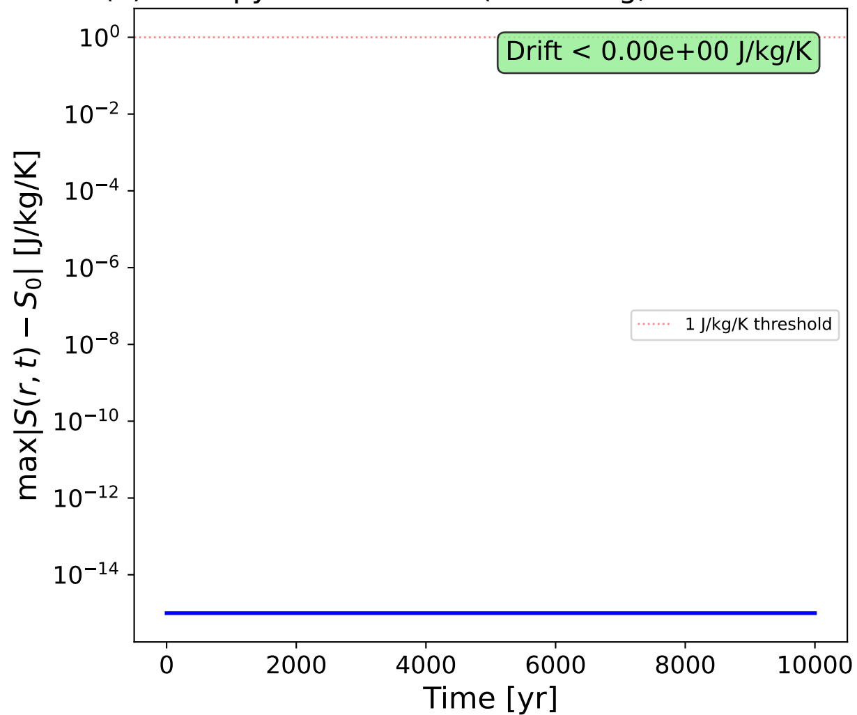
(c) Grey-body cooling ( S_0 = 10,000 J/kg/K)
