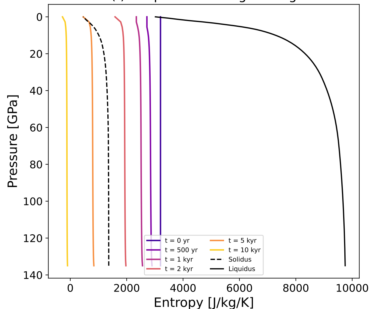
(f) P-S profiles during cooling
