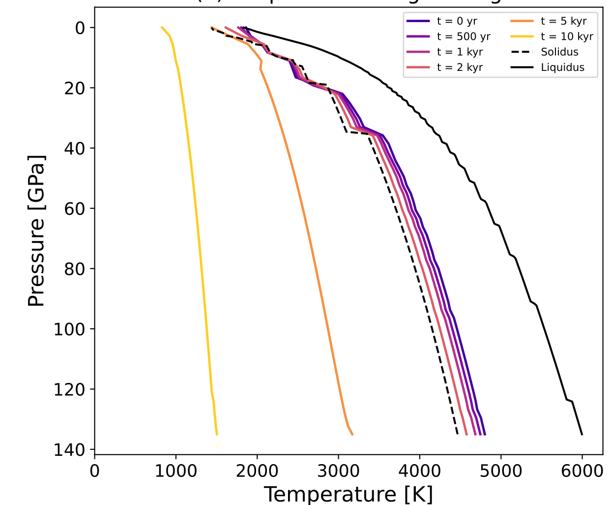
(e) T-P profiles during cooling
