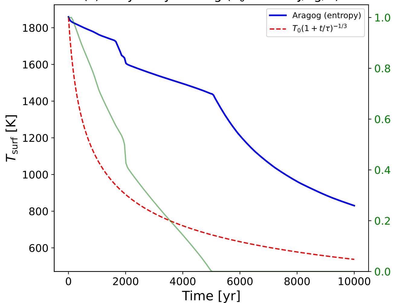
(c) Grey-body cooling ( S_0 = 3200 J/kg/K)
