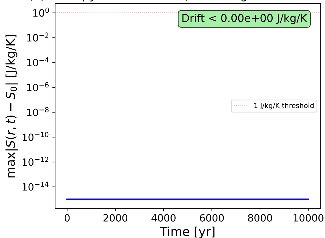
(c) Grey-body cooling ( S_0 = 10,000 J/kg/K)
