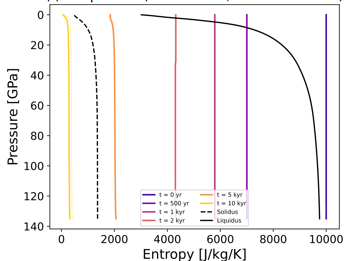
(f) P-S profiles (solid: N=50 , dashed: N=100 )
