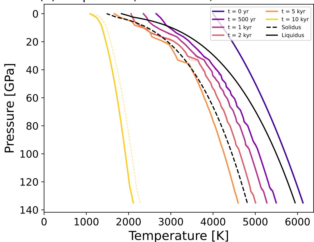
(e) T-P profiles (solid: N=50 , dashed: N=100 )
