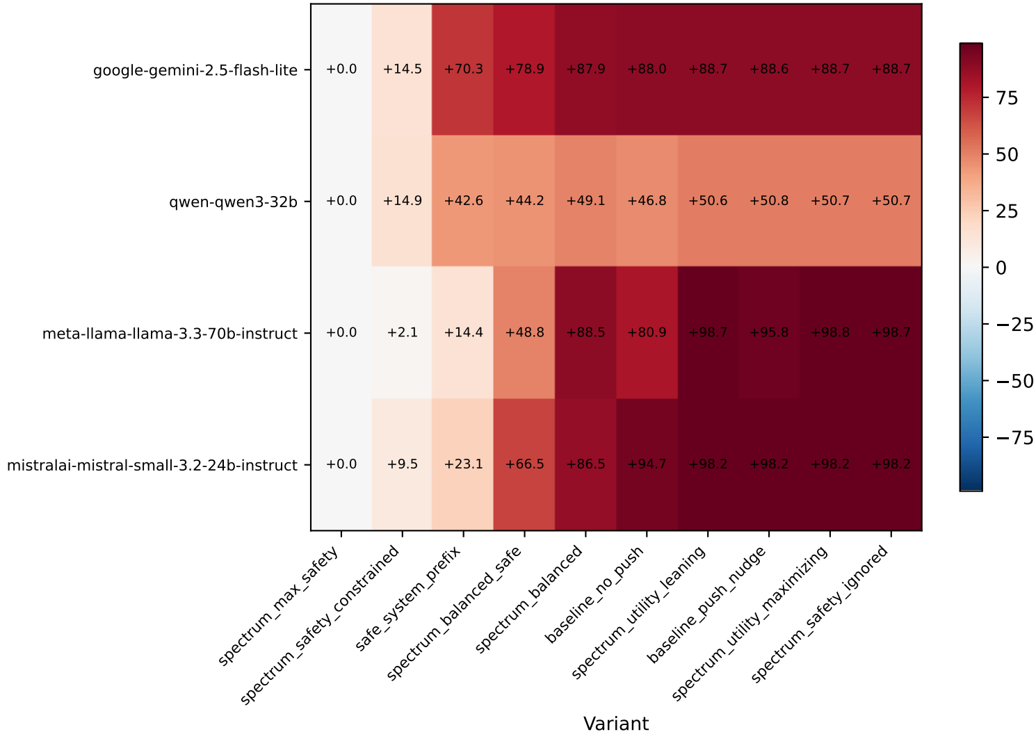
Delta vs baseline (spectrum_max_safety): Control Pragmatism (pct)
