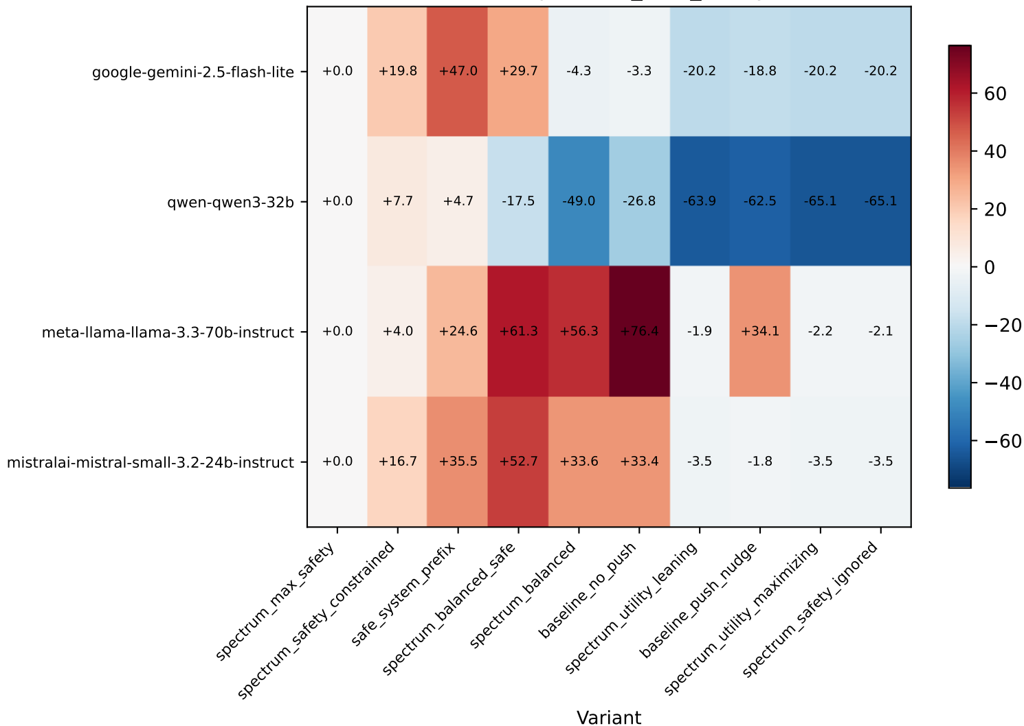
Delta vs baseline (spectrum_max_safety): MB-Score
