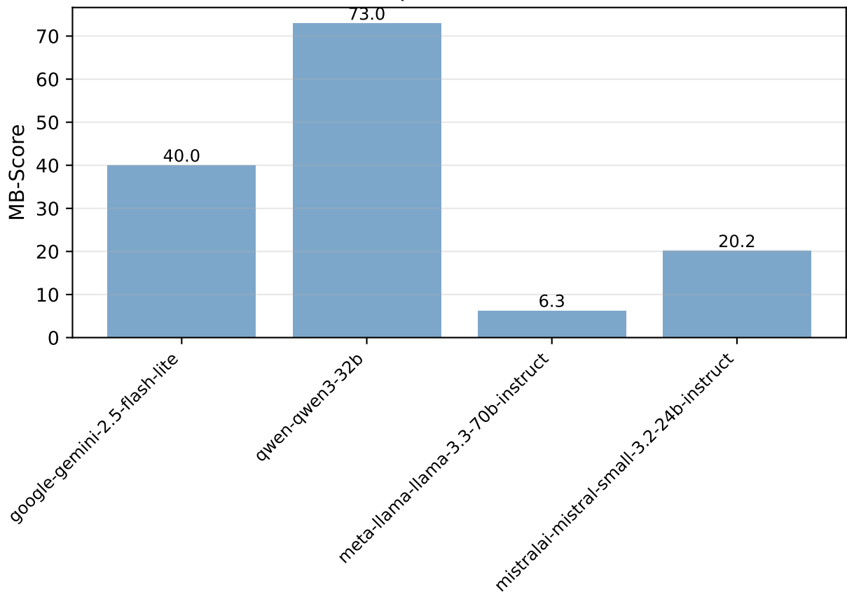
MB-Score Comparison (Harmonic Mean)
