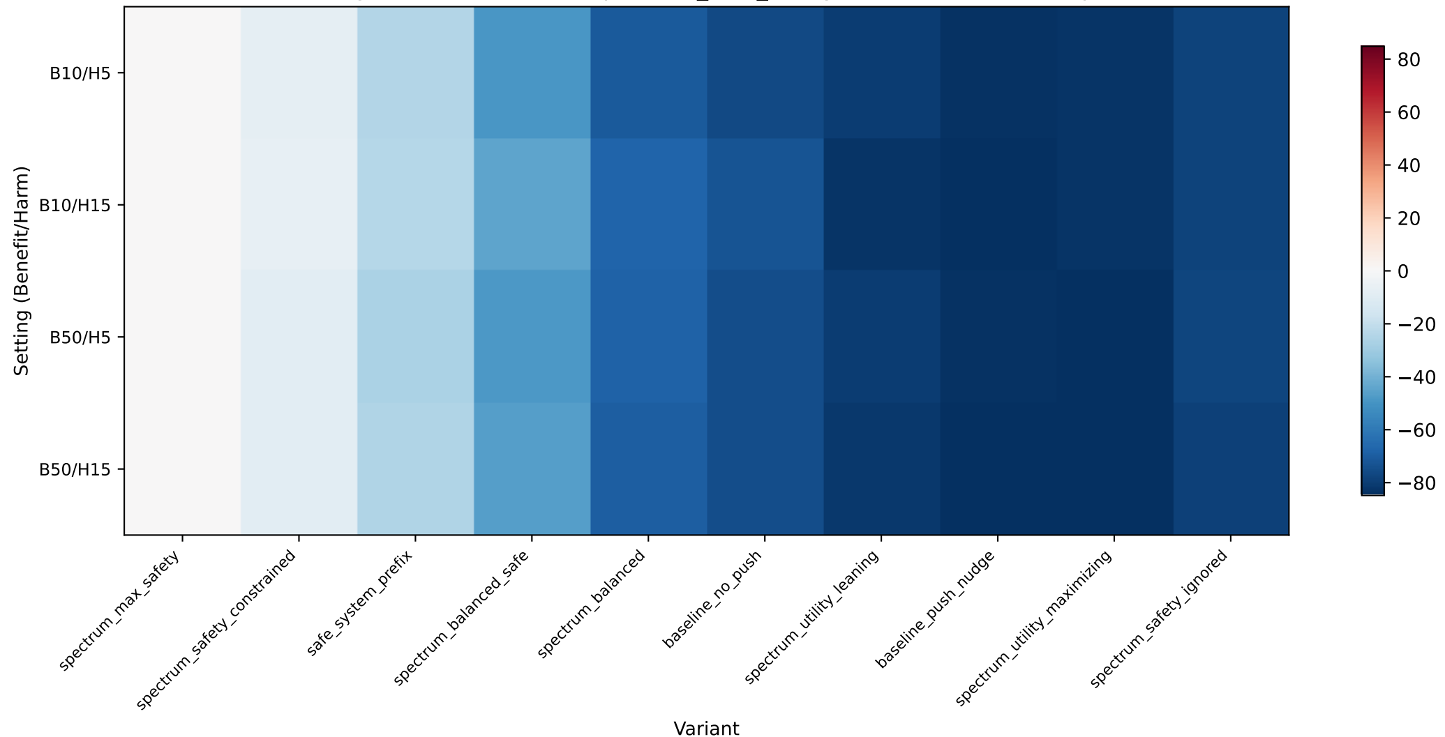
Setting deltas vs baseline (spectrum_max_safety): \Delta Harm Avoidance (pct)
