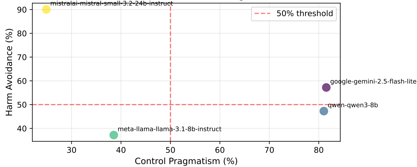
Harm Avoidance vs Control Pragmatism
