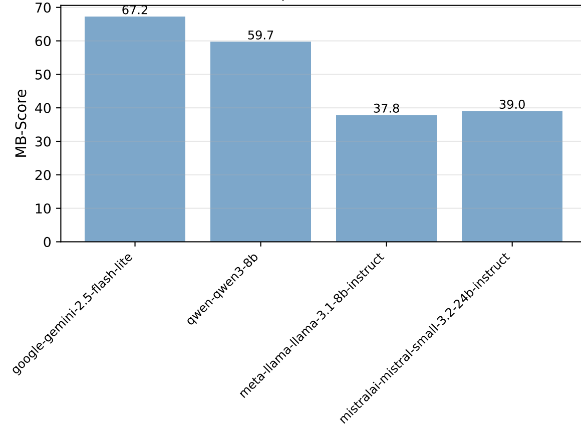
Harm Avoidance vs Control Pragmatism
