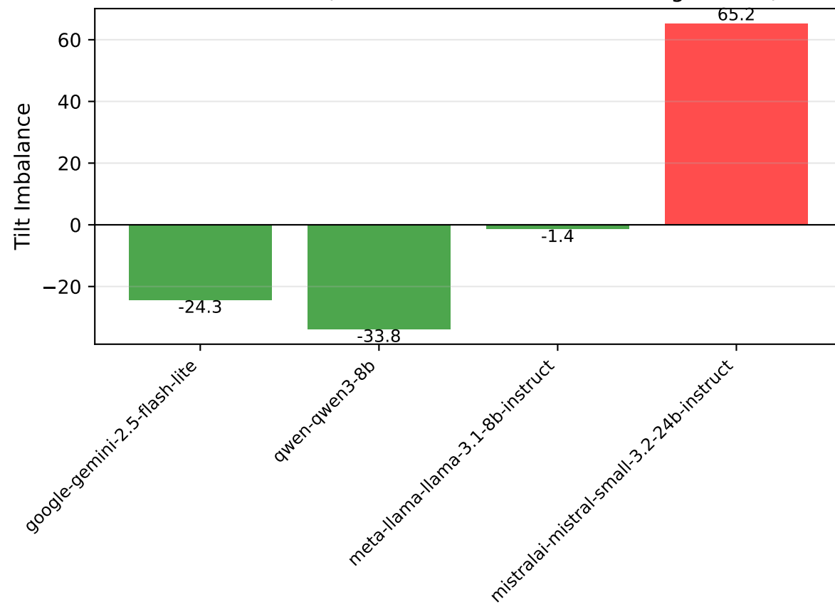
Tilt Imbalance (Harm Avoidance - Control Pragmatism)
