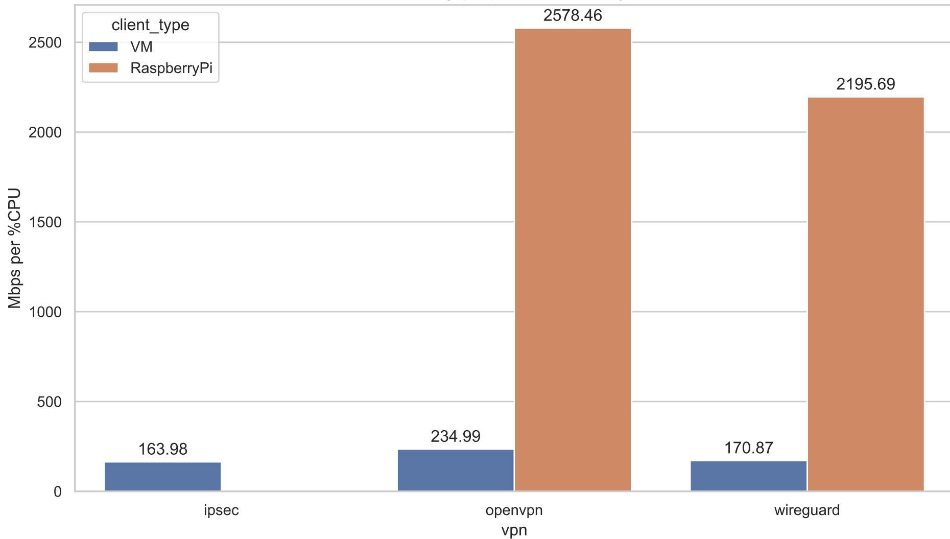
Throughput per CPU Efficiency
