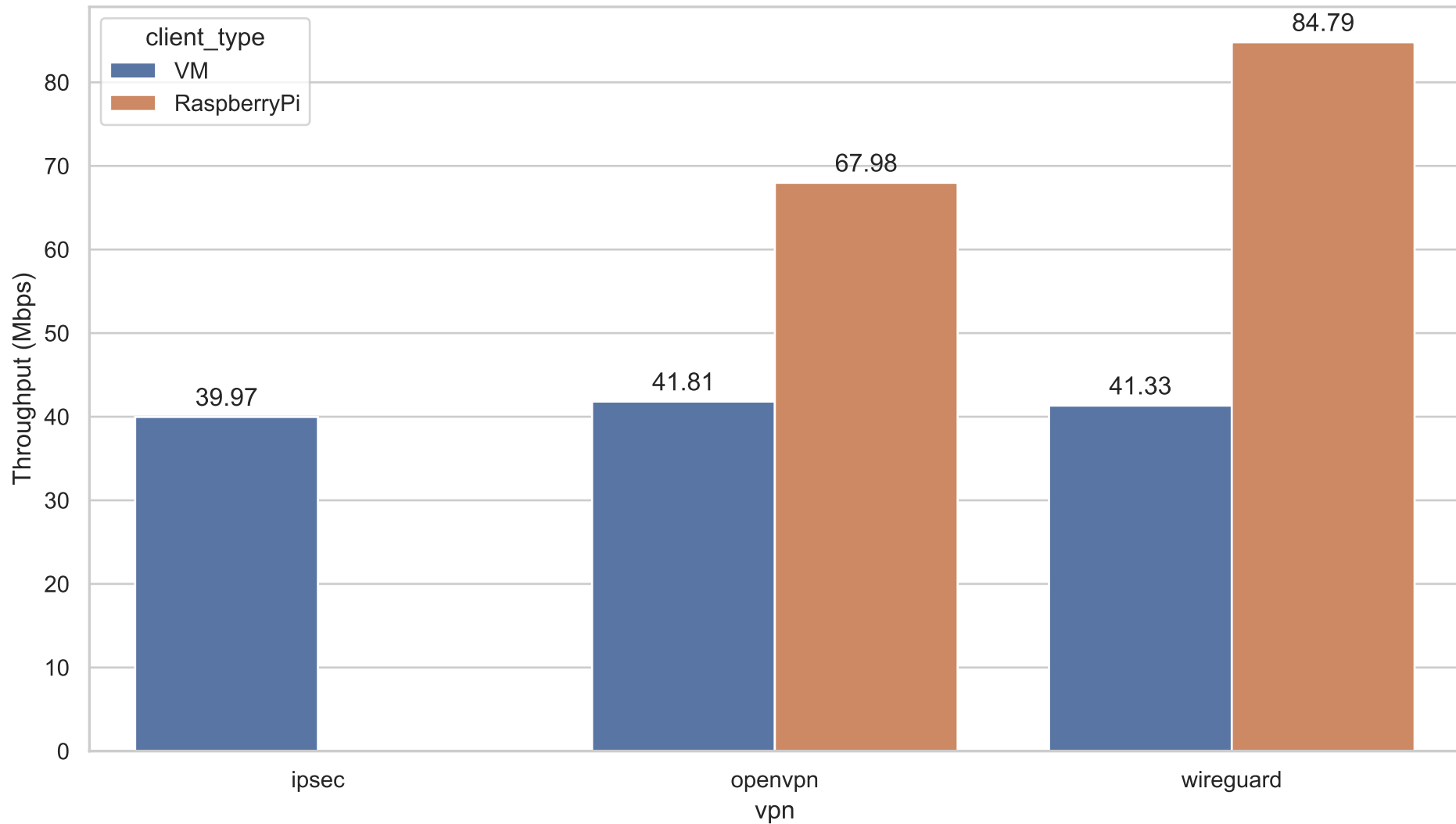
Baseline TCP Throughput
