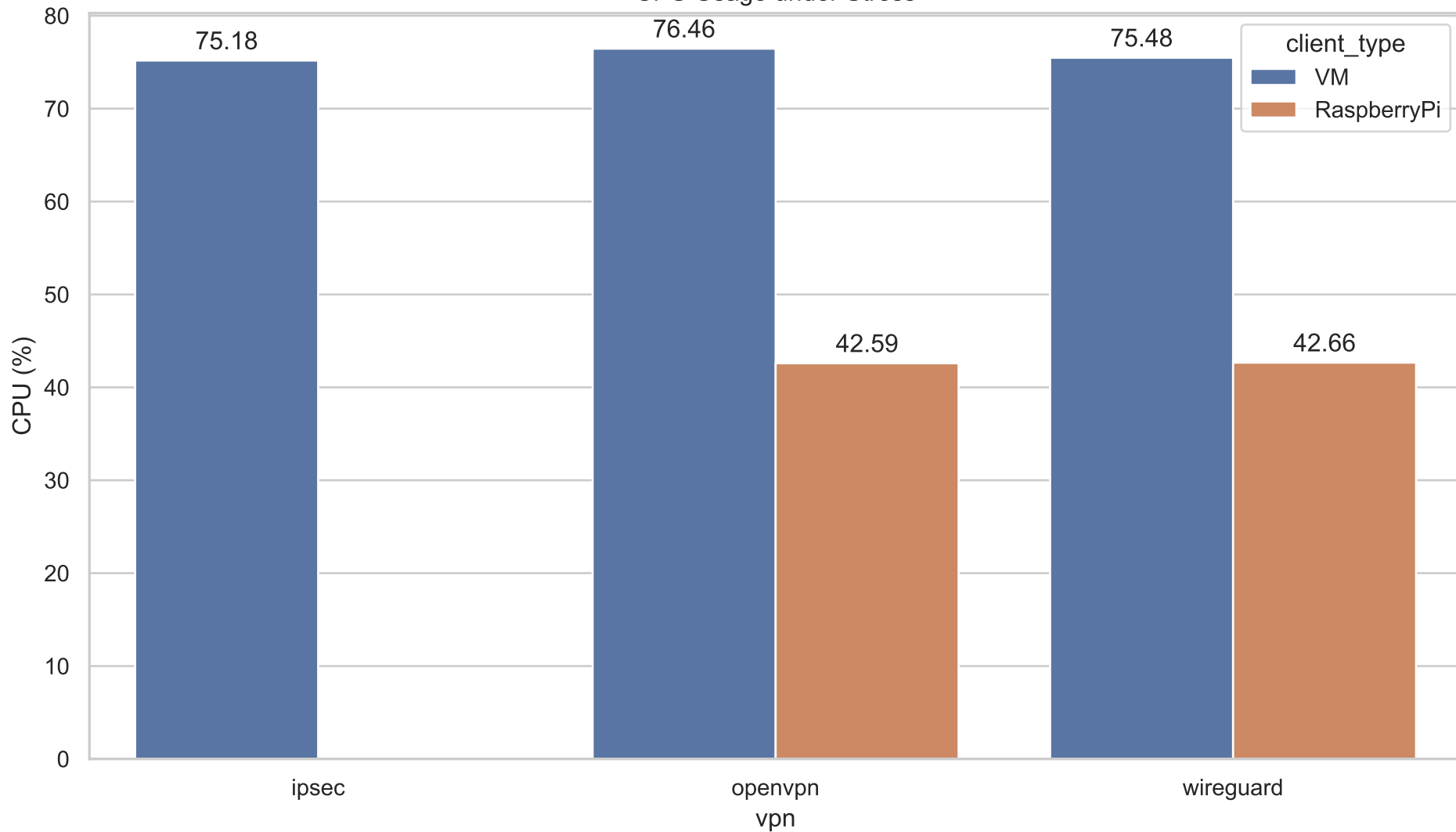
CPU Usage under Stress
