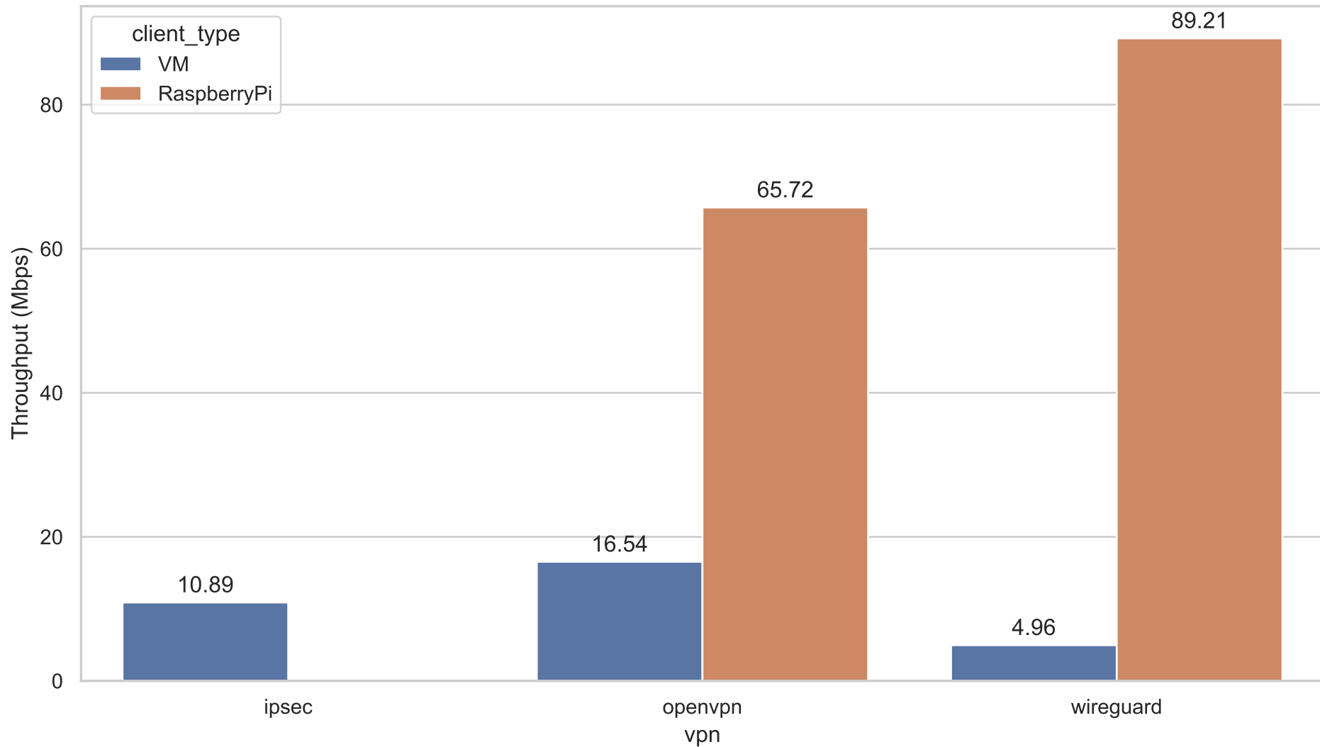
Throughput under CPU Stress
