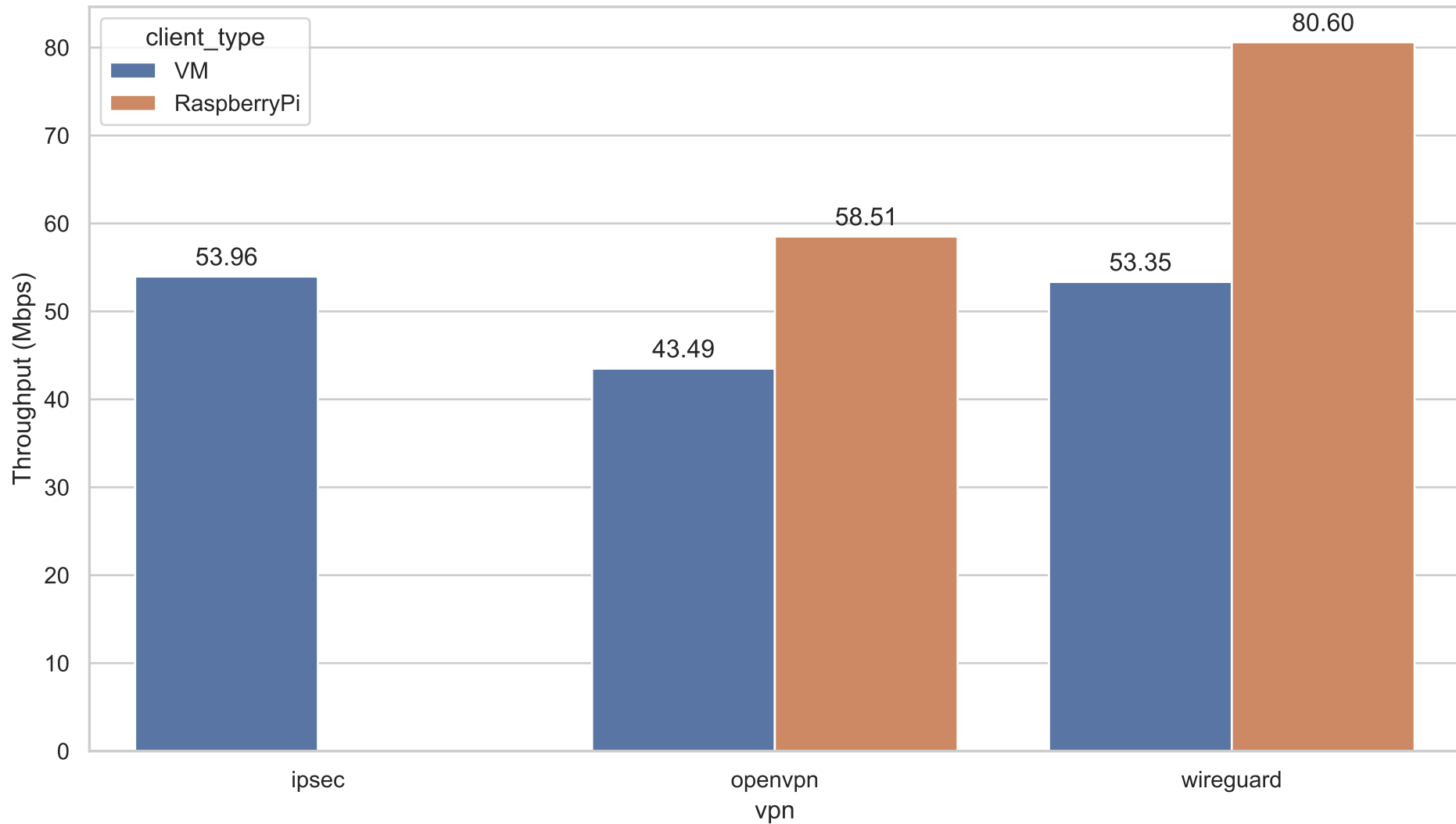
Throughput under 50 ms Latency
