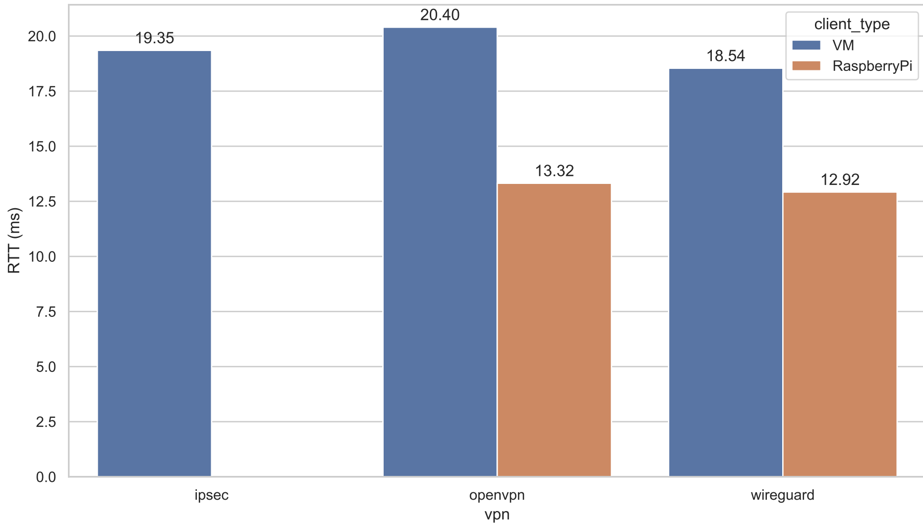
RTT under Packet Loss
