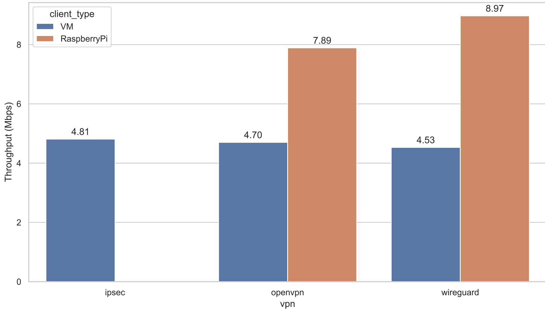
Throughput under 1% Packet Loss
