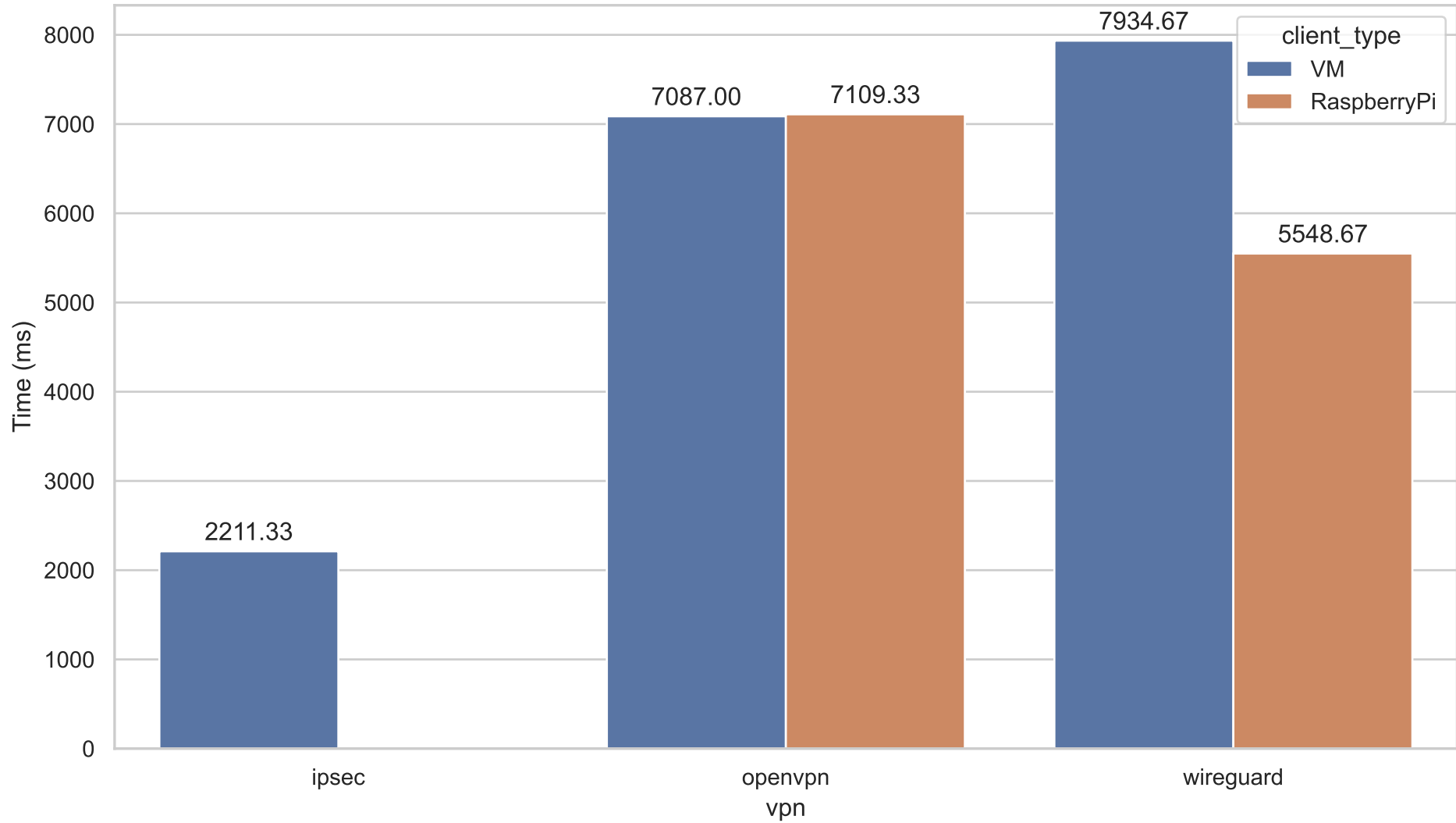
Reconnect Time (Mobility)
