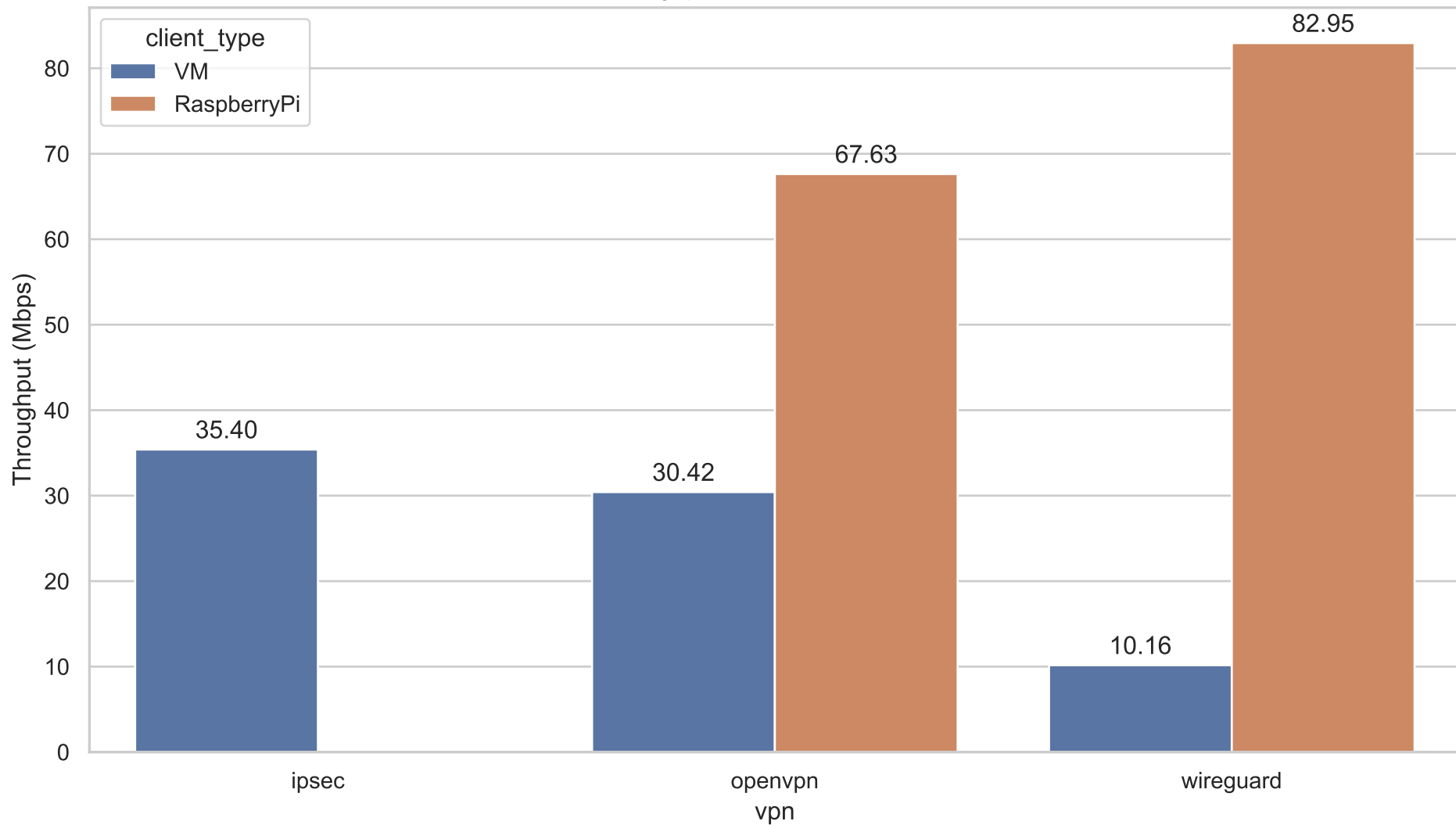
Throughput under MTU Variation
