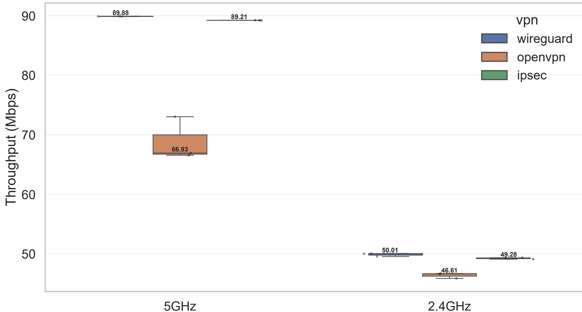
Baseline throughput: 5 GHz vs 2.4 GHz (RaspberryPi)
