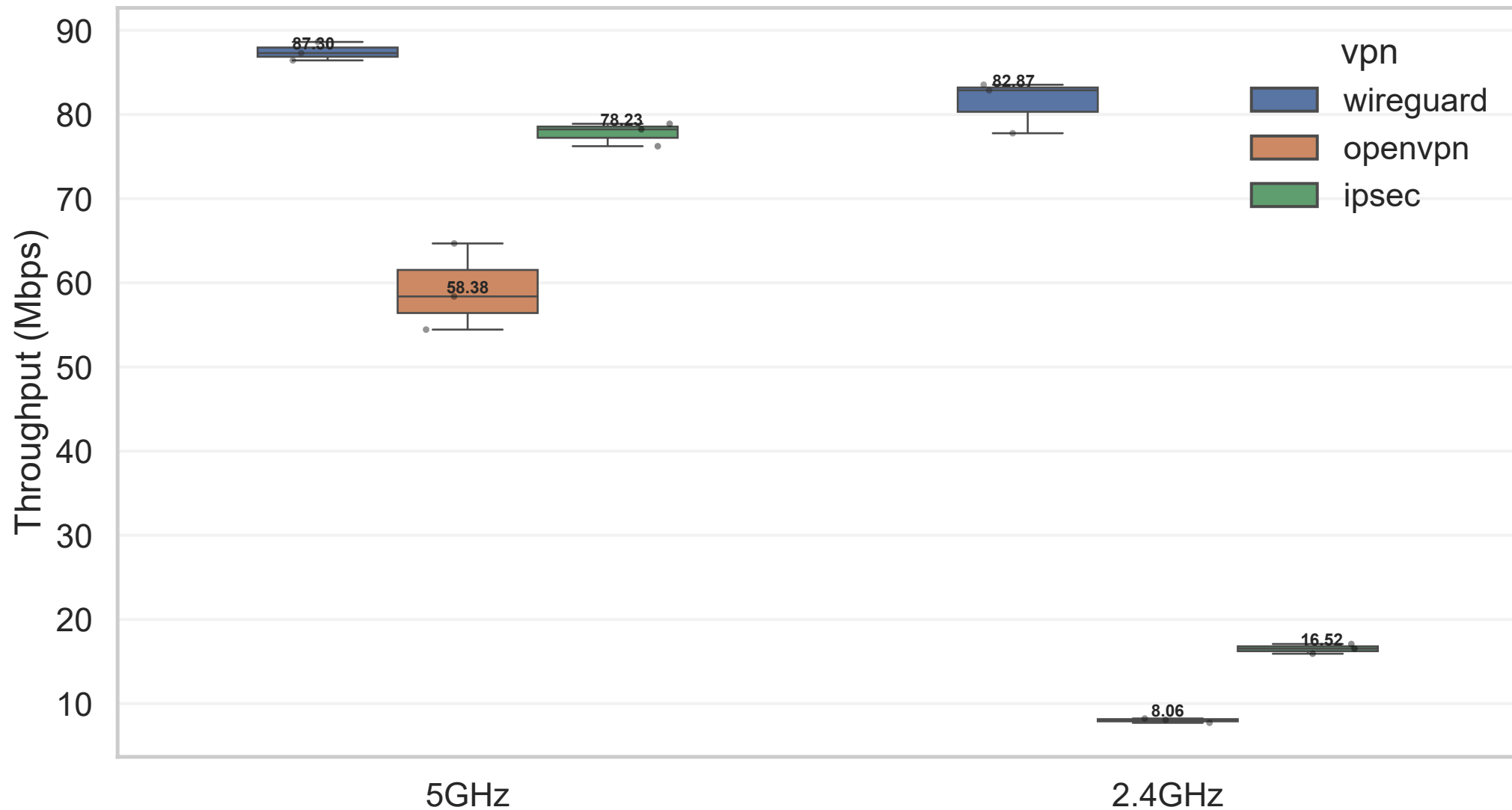
Baseline throughput: 5 GHz vs 2.4 GHz (VM)
