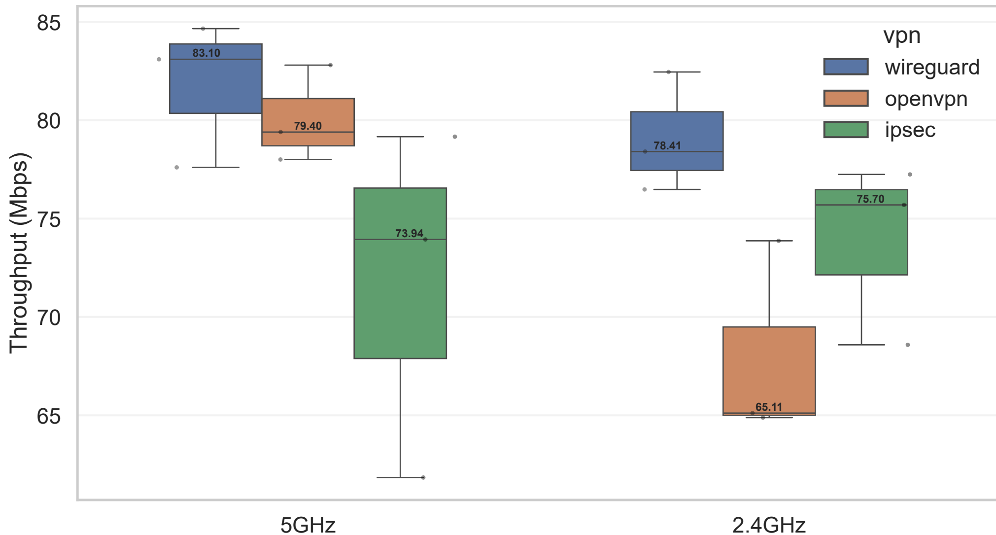
Baseline throughput: 5 GHz vs 2.4 GHz (WSL)
