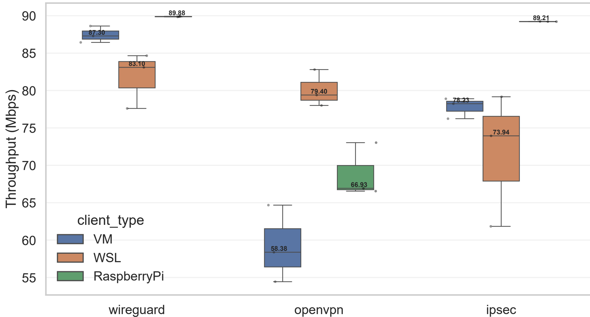
Baseline TCP throughput
