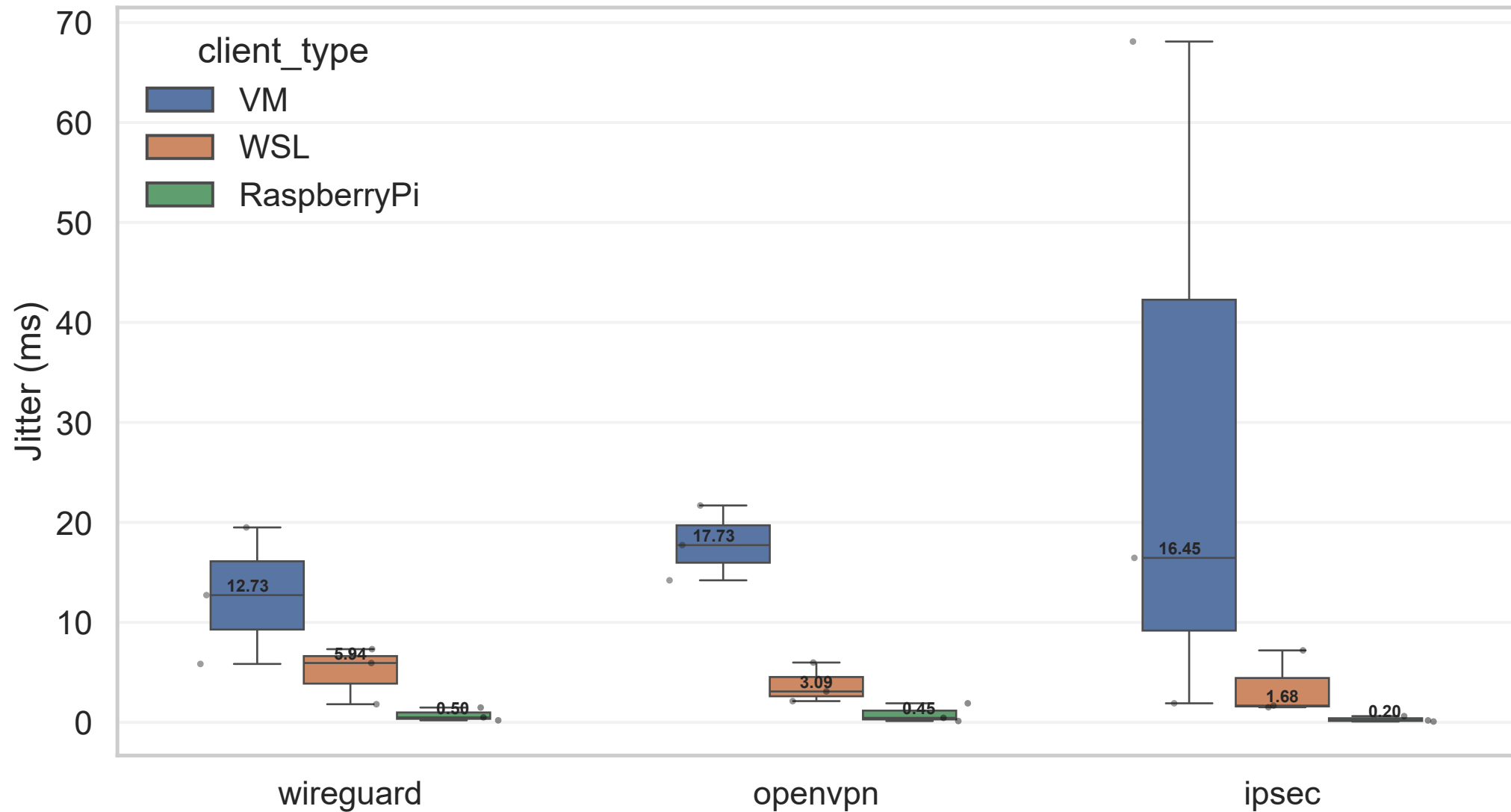
Jitter under 50 ms latency
