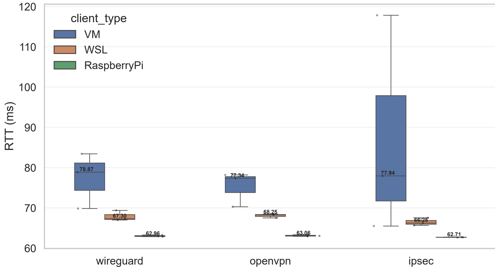
RTT under 50 ms latency
