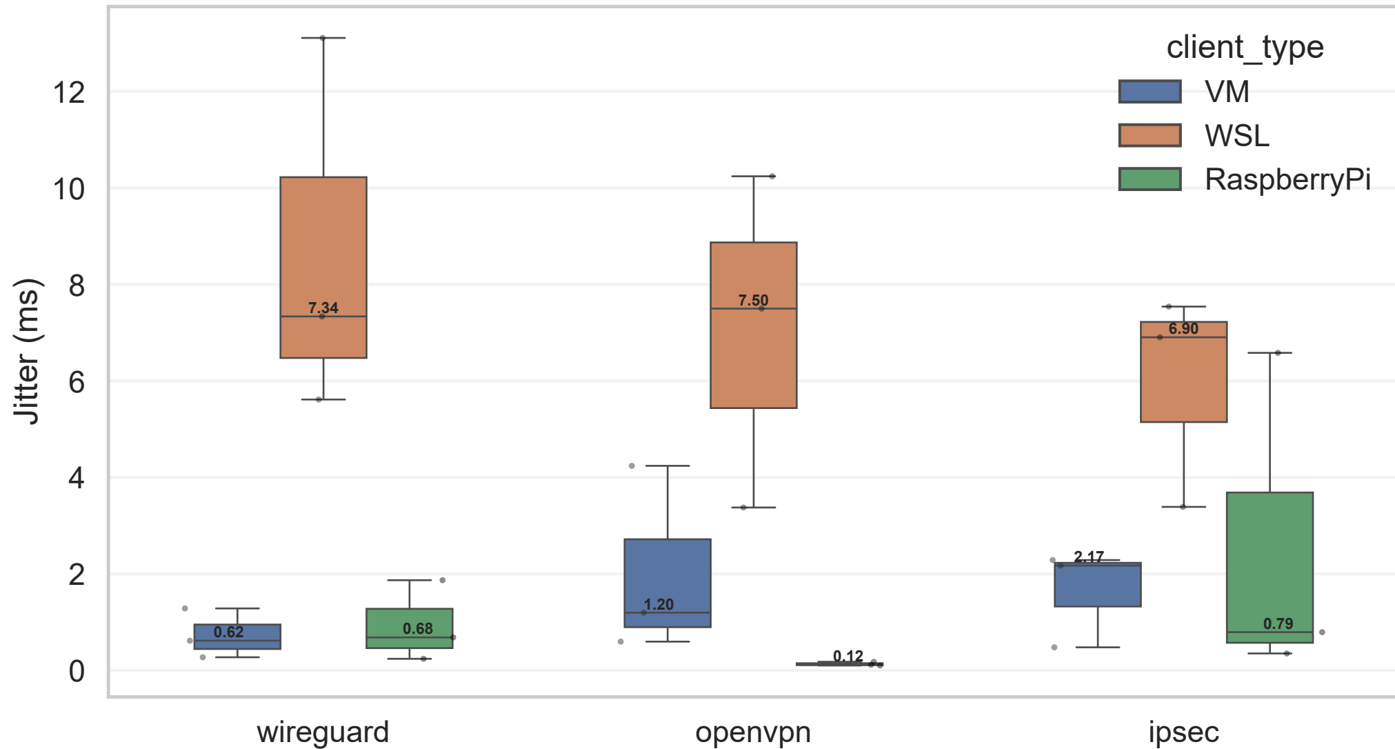
Jitter under 1% packet loss
