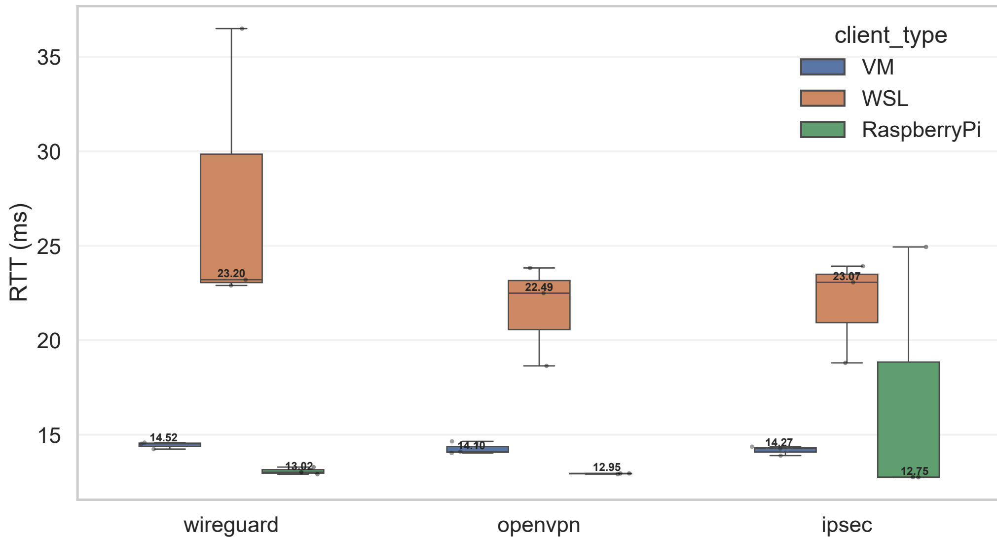
RTT under 1% packet loss
