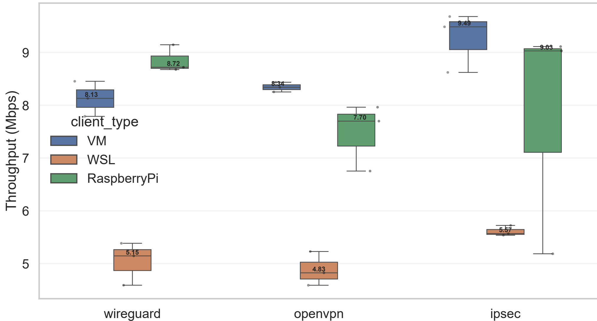
Throughput under 1% packet loss
