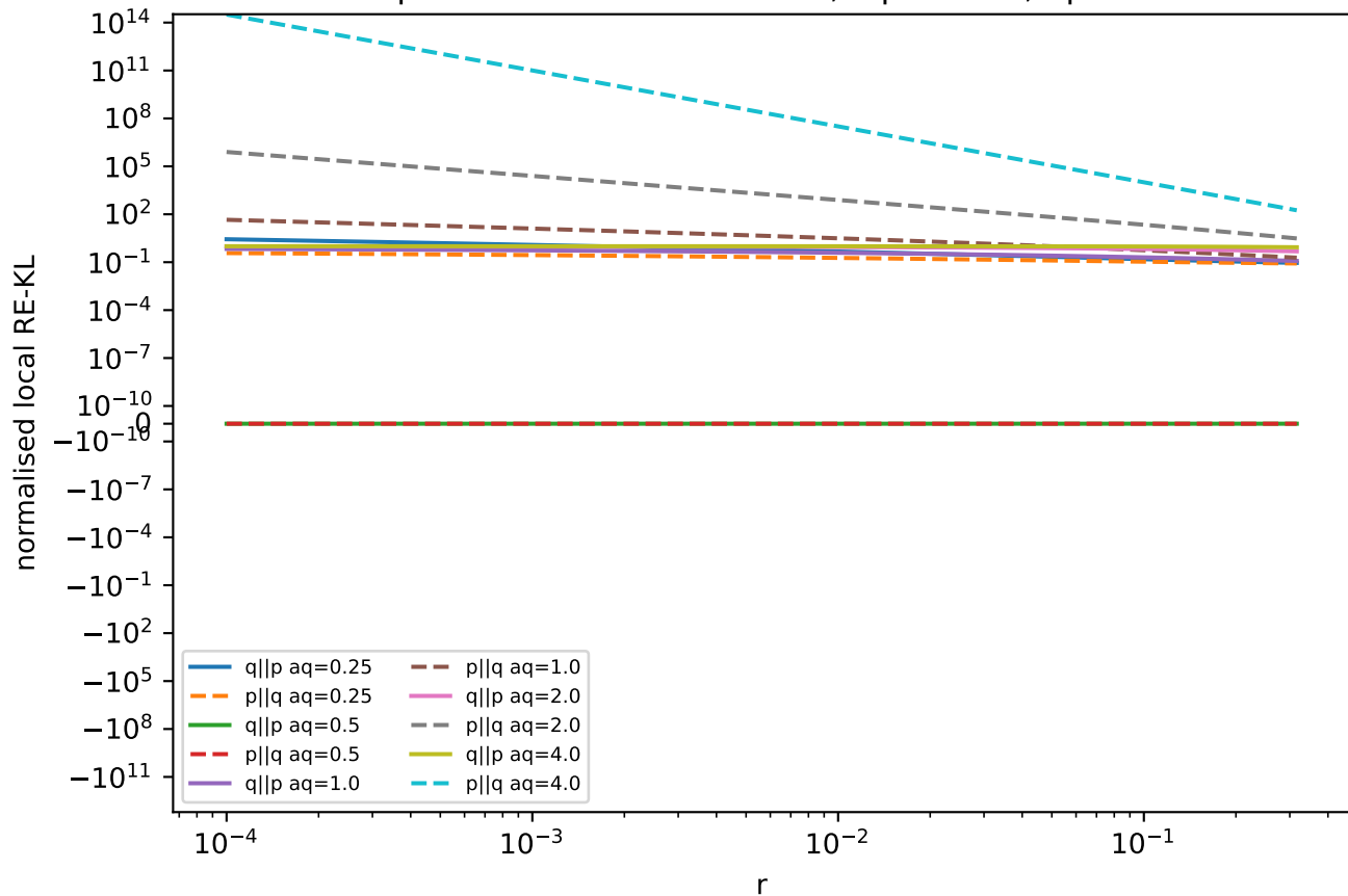
Exp3 normalised local RE-KL, alpha=0.3, ap=0.5
