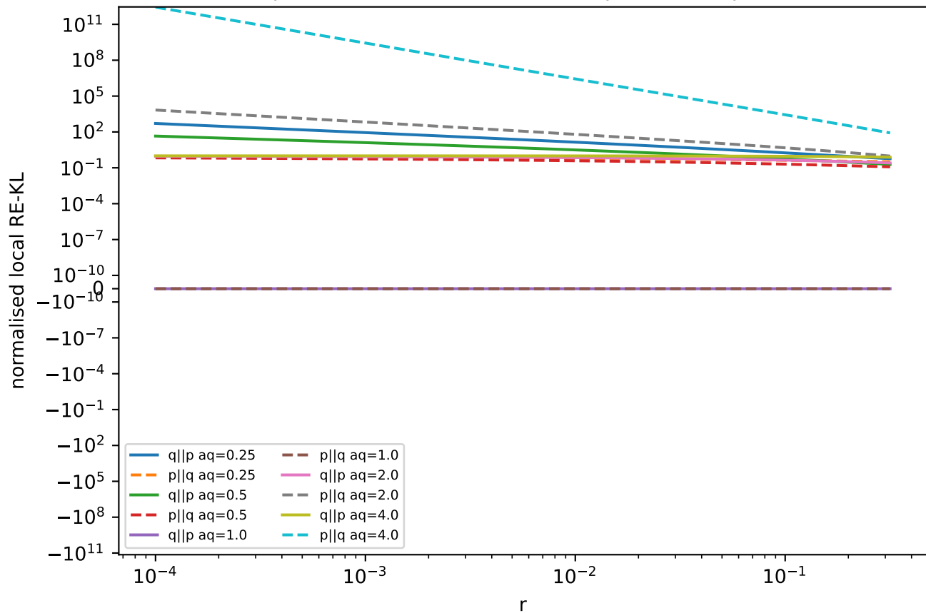
Exp3 normalised local RE-KL, alpha=0.3, ap=1.0
