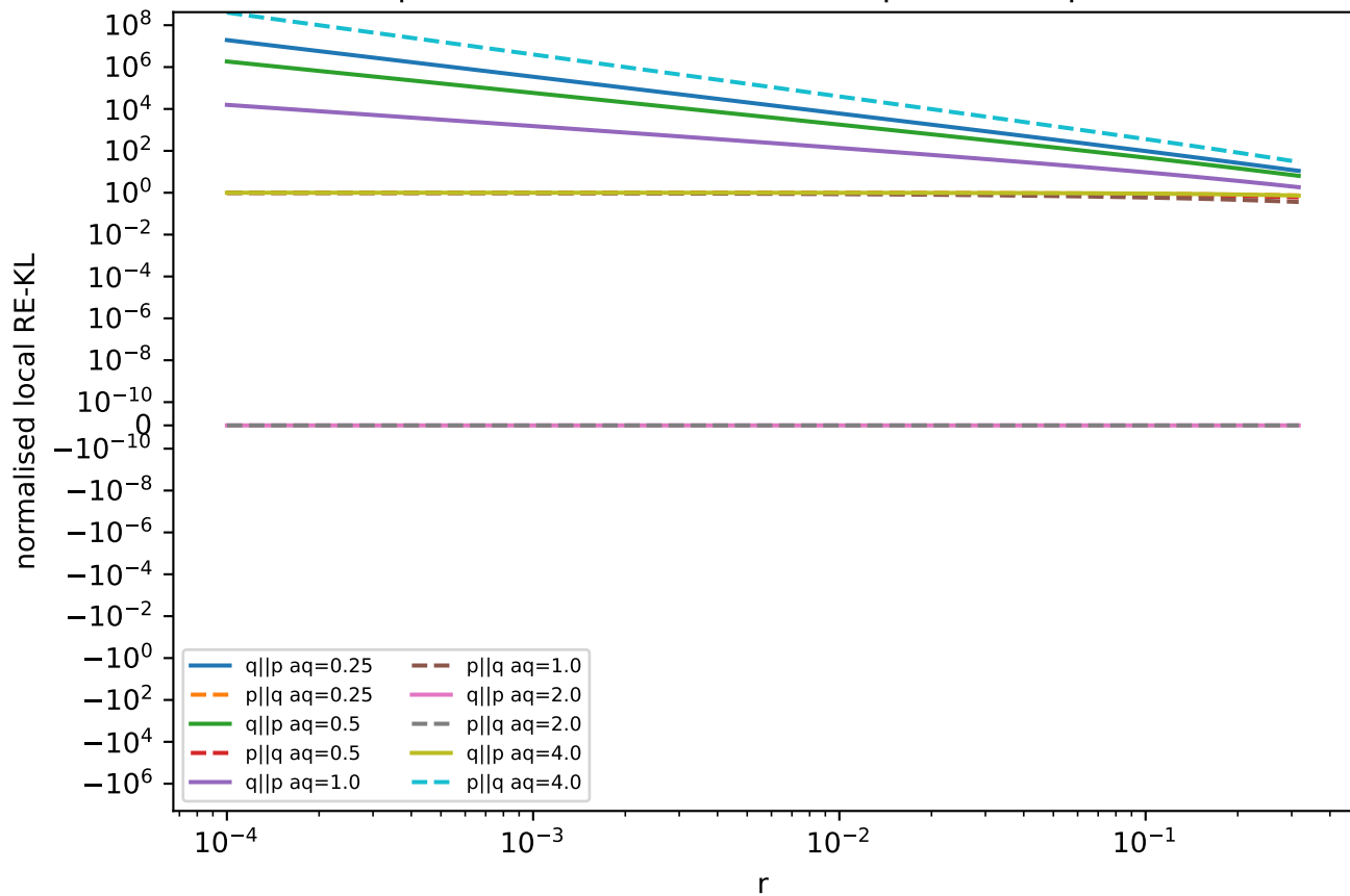
Exp3 normalised local RE-KL, alpha=0.5, ap=2.0
