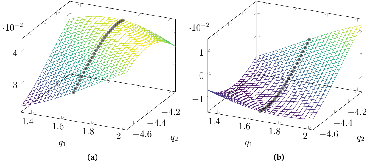
FIGURE 8 – Variation of terms from matrix (36), for q_3 = 1.5 , q_1 = 1.68 is notified by the circular black markers (a) Diagonal term on x , (b) Coupling term on x multiplied by f_z . Joint values are provided in radians.
