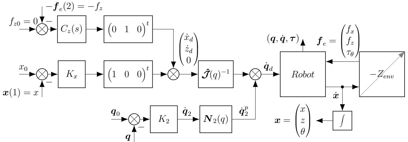
FIGURE 5 – Block diagram of the interactive robot control for a guided task on a 1 dimensional trajectory along the z axis. \mathbf{f}_e represents the interaction forces in the robot base frame, \mathbf{q} the robot joint positions, \boldsymbol{\tau} the joint torques and \mathbf{x} the robot's endpoint Cartesian coordinates. C_z = K_p + \frac{K_i}{s} is a proportional integral (PI) controller responsible for the interactive admittance control.
