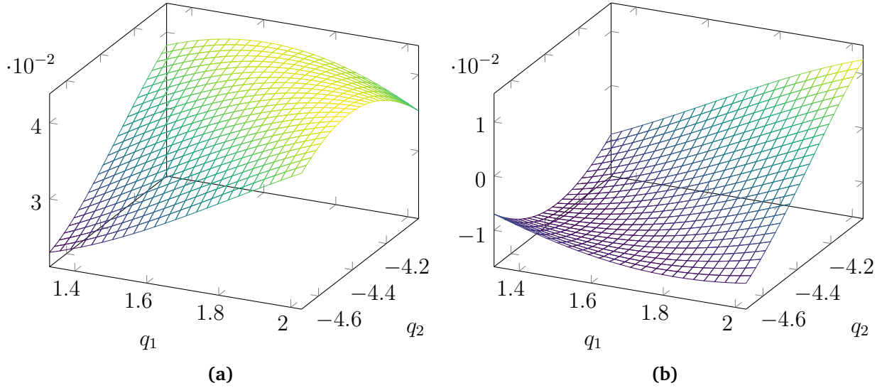
FIGURE 7 – Variation of terms from matrix (29), for q_3 = 1.5 (a) Diagonal term on x , (b) Coupling term on x multiplied by f_z . Joint values are provided in radians.
