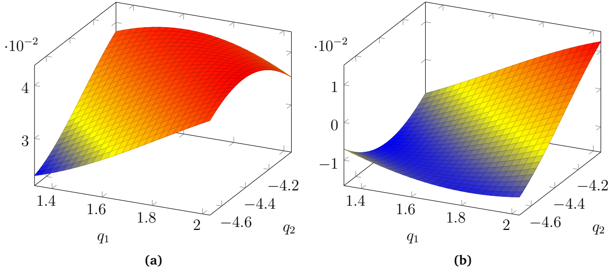
FIGURE 7 – Variation of term of the matrix (29), for q_3 = 1.5 (a) Diagonal term on x (b) Coupling term on x multiplied by f_z . Joint values are given in radians.
