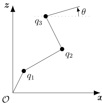
FIGURE 4 – Robot plan redondant
