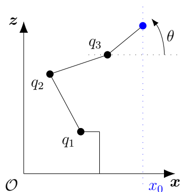
FIGURE 1 – Robot plan redondant
